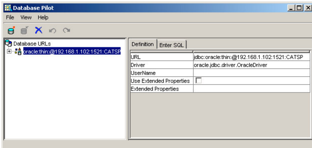
Figure 19. Entering other properties of the datasource
