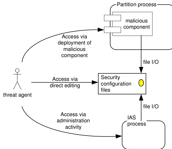
Figure 9. Access paths to BES Security Configuration Files
